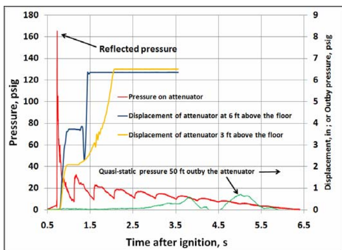
Figure 9. Reflected explosion pressure inby the Attenuator (A-375) and the quasi-static pressure 15 m (50 ft) outby the Attenuator (A-453) during the first test (LLEM Test #525). Displacement of the Attenuator as measured with LVDTs is also shown.
