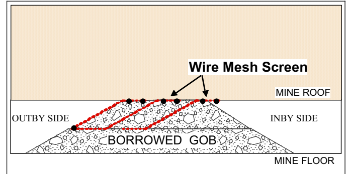
Figure 2. The “fully-stowed” alternate Attenuator design with sections of corrosion resistant wire roof mesh to provide confinement and passive reinforcement to minimize material erosion during the pressure blow down. This design was tested and evaluated in full-scale explosion tests at the NIOSH Lake Lynn Experimental Mine, but without the wire mesh screen.
