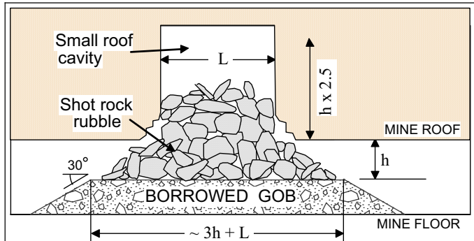
Figure 1. The “shot-rock” optimum Attenuator design where a section of the mine roof is shot down with explosives using holes drilled prior to placement of an optional foundation layer of borrowed gob material.
